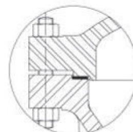
BODY-BONNET JOINT
