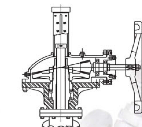
WITH ENCLOSED TYPE BEVEL GEAR ARRANGEMENT
