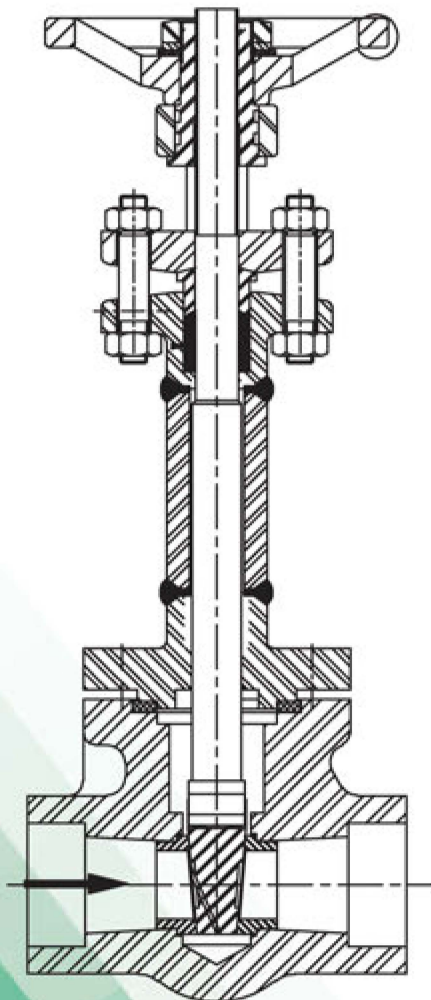
GATE VALVE
