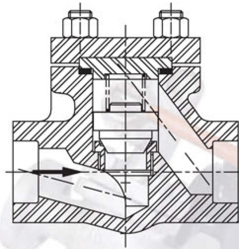
CHECK VALVE
